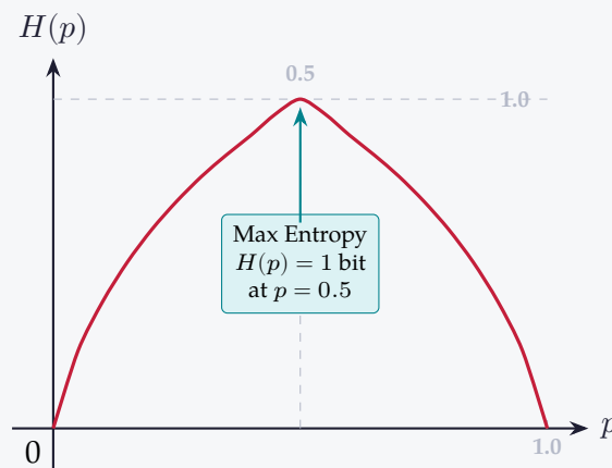
Binary Entropy Function H(p) vs p
